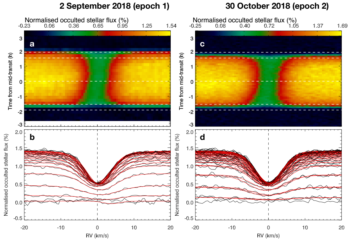
Extended Data Figure 4 | Doppler shadow of WASP-76. a,c, Local stellar CCFs behind the planet represented as a function of time for epoch 1 (a) and epoch 2 (c). The horizontal dashed lines represent (from bottom to top) the 2 nd contact, mid-transit and 3 rd contact. b,d, 1D view of the local stellar CCFs (black lines) with their Gaussian fits (red curves).
