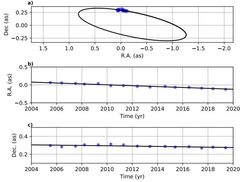
Fig. 6 Keplerian orbit of the D9 system. In subplot (a), the projected on-sky trajectory of the D9 binary system is shown. Subplot (b) and (c) shows the R.A. and DEC. position as a function of time. In subplot (b) and (c), the low proper motion is eminent. Every blue-colored data point in this figure is related to one observational epoch. From this plot and the related inclination of i_{\text{orb}} = (102.55 \pm 2.29)^\circ , it is suggested that the trajectory of the binary system is close to edge-on. The size of the blue data points are related to the astrometric uncertainty of \pm 0.006 as.
