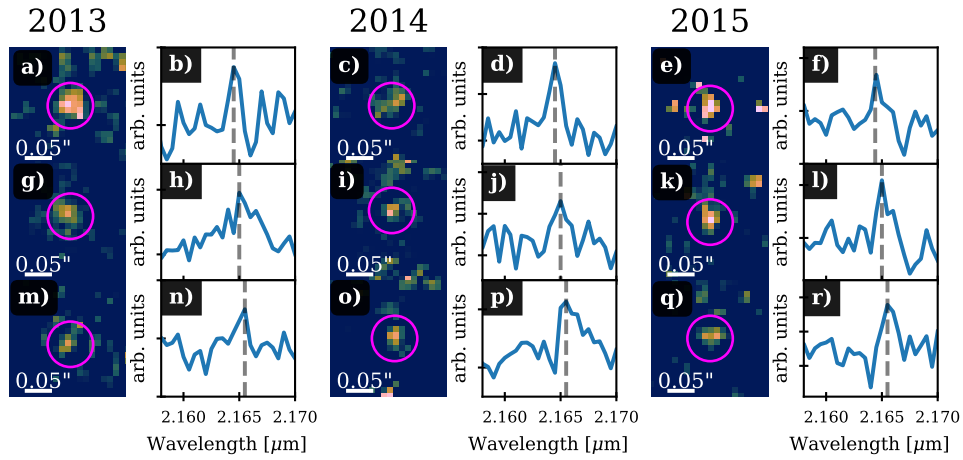
Fig. 7 Doppler-shifted \text{Br}\gamma line of D9 and the related line maps representing the magenta-marked emission. Subplots (a), (c), (e), (g), (i), (k), (m), (o), and (q) show SINFONI line maps of the binary system D9. In these subplots, D9 is marked with a magenta-colored circle. In subplots (b), (d), (f), (h), (j), (l), (n), (p), and (q), we apply a local background subtraction of the surrounding gas to the presented spectra. The successful subtraction of the background is evident in the absence of the prominent \text{Br}\gamma peak at 2.1661\mu\text{m} [101, 102]. The shown spectra shows the evolution of the line over one year. The normalized \text{Br}\gamma velocity v_{\text{norm}} in 2013 is approximately 66 km/s (b), 3 km/s (h), and -72 km/s (n). In 2014, v_{\text{norm}} is about 68 km/s (d), 3 km/s (j), and -71 km/s (p). In 2015, we estimate v_{\text{norm}} to be around 72 km/s (f), 1 km/s (l), and -67 km/s (r).
