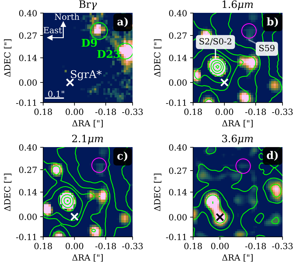
Fig. 1 Detection of the D9 system close to Sgr A* in 2019. Subplot (a) shows the Doppler-shifted Br \gamma line map extracted from the H+K SINFONI data cube with a corresponding wavelength of 2.1646 \mu\text{m} (vacuum wavelength 2.1661 \mu\text{m} ). Subplot (b) and (c) shows the near-infrared H ( 1.6 \mu\text{m} ) and K ( 2.1 \mu\text{m} ) band data observed with SINFONI. Subplot (d) denotes the mid-infrared L ( 3.76 \mu\text{m} ) band observation carried out with NIRC2. Sgr A* is marked with a \times , D9 is encircled in every plot. Due to its main sequence character, the marked close-by star S59 can only be observed in the H and K bands. On the contrary, the brightest K band source of the S cluster, S2/S0-2 can be observed in every shown infrared band. To increase contrast, an image sharpener is applied suppressing expansive point spread function (PSF) wings. To emphasize the astrometric robustness of the image sharpener, we adapt the lime-colored contour lines from the non-sharpened data. The contour line levels in panel (b) are at 10%-80% of the peak intensity of S2, increasing in 5% steps. In panel (c), the contour lines are set at 20%-100% of the peak intensity of S2, separated by 10%. For panel (d), the contour lines are set to 85%, 90%, 95%, and 100% of the peak intensity of S2. The labels of the axis indicate the distance to Sgr A* located at \Delta\text{RA}=0.00'' and \Delta\text{DEC}=0.00'' . In any plot shown, north is up, and east is to the left.
