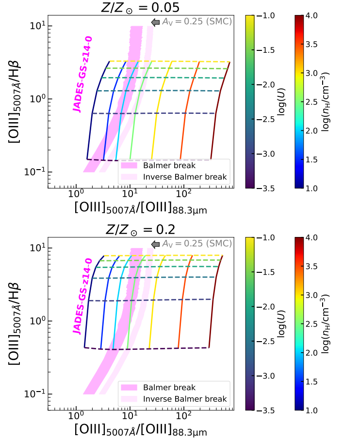
Fig. 4: [\text{O III}]5007\text{\AA}/[\text{O III}]88\mu\text{m} versus [\text{O III}]5007\text{\AA}/\text{H}\beta diagram. Top and bottom panels show model grids computed with CLOUDY with metallicities Z/Z_{\odot} = 0.05 to Z/Z_{\odot} = 0.2 , respectively. Each model grid spans a range of ionization parameters ( -3.5 \leq \log U \leq -1 ) and hydrogen densities ( 10 \text{ cm}^{-3} \leq n_{\text{H}} \leq 10^4 \text{ cm}^{-3} ) in steps of 0.5 dex. Details on model parameters are provided in Tab. 1. The magenta-shaded regions show the plausible attenuation-corrected line ratios for JADES-GS-z14-0 inferred from observations by JWST/MIRI and ALMA. The dark regions report the range of line ratios assuming that the MIRI excess is only due to the optical line. The light regions illustrate the range of line ratios in the case the stellar age is 1 Myr and there is an inverse Balmer break in the spectrum. The gray arrow represents a reddening vector with A_{\text{V}} = 0.25 assuming the nebular dust attenuation follows an average SMC extinction curve.
