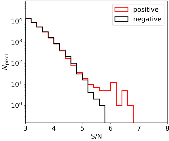
Fig. A.1: Statistics of positive and negative peaks from natural-weighted spectral cubes, collapsed with various velocity bin sizes at 30\text{--}170\text{ km s}^{-1} . The maximum \text{S/N} = 6.67 is seen at the centroid of JADES-GS-z14-0 at 223.524\text{ GHz} with a velocity bin size of 130\text{ km s}^{-1} , for which we interpret as an [O III] 88\mu\text{m} line detection at z = 14.1796 . This is much more significant than the strongest negative peak seen in the spectral cube ( -5.7\sigma ). Therefore, we conclude the fidelity of ALMA line detection.
