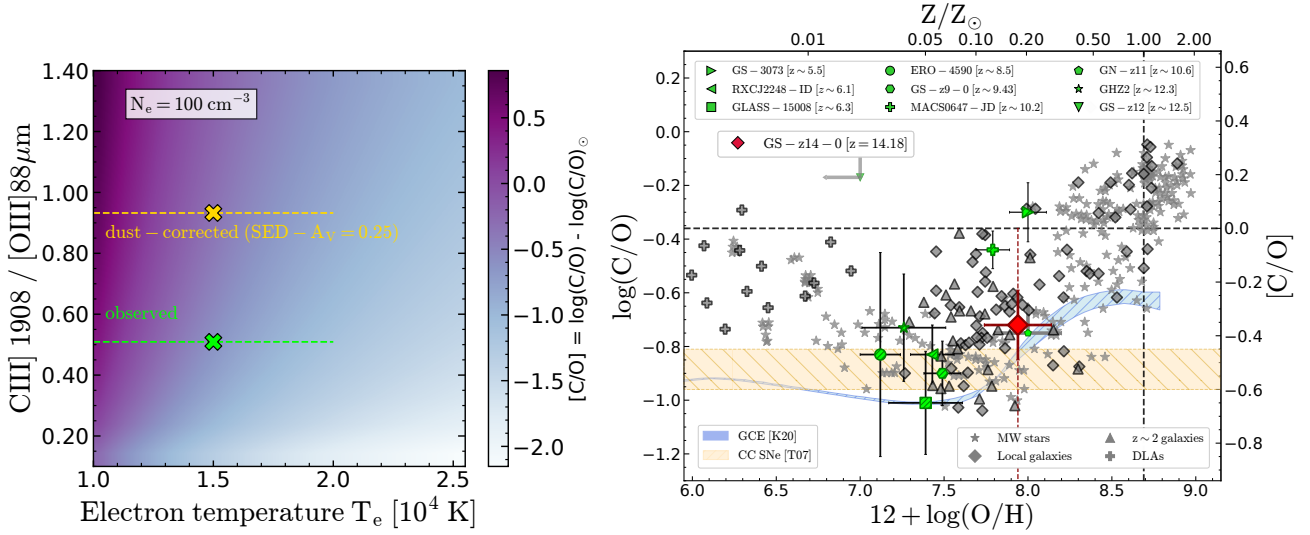
Fig. 7: Carbon-over-oxygen abundance for JADES-GS-z14-0. The left-hand panel shows how the final inferred C/O value changes as a function of the \text{C III]}/[\text{O III}]88\mu\text{m} line ratio and of the electron temperature, T_e , under our fiducial assumption of N_e=100 \text{ cm}^{-3} . The observed and dust-corrected \text{C III]}/[\text{O III}]88\mu\text{m} ratios for JADES-GS-z14-0 are marked in green and yellow, respectively. In the right-hand panel, we report our fiducial C/O measurement for JADES-GS-z14-0 on the C/O vs O/H diagram. The oxygen abundance is inferred from the best-fit PROSPECTOR metallicity reported in Table 2. The C/O value measured in JADES-GS-z14-0 is consistent with pure enrichment from core-collapse Supernovae. We also report for comparison a sample of C/O measurements from JWST compiled from the literature, namely GS-z12 ( z = 12.5 ; D'Eugenio et al. 2024b), GHZ2 ( z = 12.34 ; Castellano et al. 2024), GN-z11 ( z = 10.6 ; Cameron et al. 2024), MACS0647-JD ( z = 10.2 ; Hsiao et al. 2024b), GS-z9-0 ( z = 9.4 ; Curti et al. 2024), ERO-4590 ( z = 8.5 ; Arellano-Córdova et al. 2022), RXCJ2248-ID ( z = 6.11 ; Topping et al. 2024), GLASS-150008 ( z = 6.23 ; Jones et al. 2023), GS-3073 ( z=5.5 ; Ji et al. 2024). The C/O vs O/H pattern predicted by Galactic Chemical Evolution models of Kobayashi et al. (2020) is shown in blue, whereas the C/O range allowed by the CC-SNe yields from Tominaga et al. (2007) is marked by the golden region.
