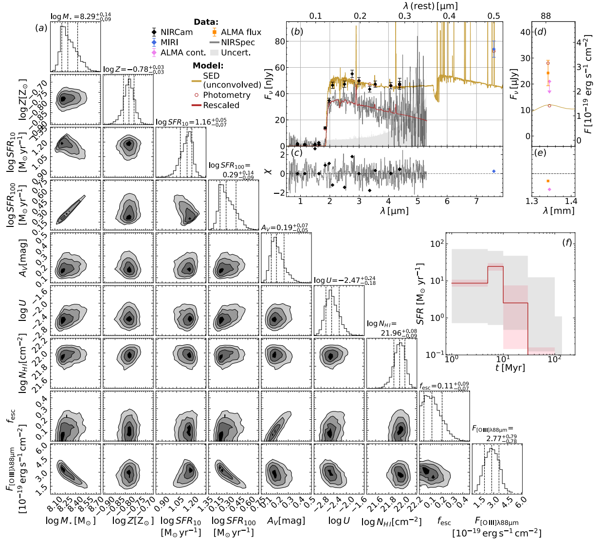
Fig. 5: Summary of prospector SED model. Panel a . Triangle diagram with the marginalized posterior distribution over a subset of the model-free or dependent parameters (see Table 2 for a description of the parameters and their probability prior). Panel b . SED, including wide- and medium-band measured flux densities (diamonds), the spectrum (grey line with grey region as the uncertainty). NIRCam, MIRI and ALMA data are in black, blue and pink, respectively. Model predictions are red circles (flux densities) or the red line (spectrum). The sand-coloured line is the model SED without convolving to the spectral resolution for the data. Panel c . Model residuals normalised by the uncertainties. Panel d . Same as panel b , but for the FIR region. The orange square is the ALMA [O III] flux. Panel e . Same as panel c , but for the FIR region. Panel f . Star-formation history (red), with the prior probability in grey.
