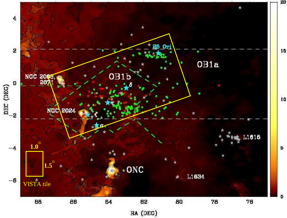
Figure 1: The yellow tilted square indicates the proposed VISTA survey area. The size is \sim 30 square degree and it will be mapped with 20 contiguous VISTA tiles. The figure has been adapted from Briceño (2008), with the underlying colour map showing the dust emission map of Schlegel et al. (1998), represented in false color calibrated to E(B - V) reddening in magnitudes. The three Orion belt stars, and \sigma Ori and 25 Ori are plotted as large cyan starred symbols. Other symbols are pre-main-sequence stars: weak-line TTauri stars (green dots), classical TTauri stars (red dots) from Briceño et al. (2005, AJ, 129, 097). PMS stars identified by Alcalá et al. (2004) and in Herbig & Bell (1988) are shown as grey stars. The horizontal dashed lines indicate the limits of the Briceño et al. (2005) survey. The green dashed lines show the boundaries of Ori OB1a and OB1b association from Warren & Hesser (1977).
