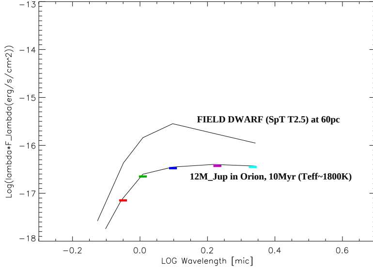
Figure 2: The observed SED of an old field T-dwarf (Chiu et al. 2008, MNRAS 385, L53) compared to the SED of a 12M_{Jup} mass object of age 10Myrs, at the distance of 400 pc, and seen through A_V = 1 mag (based on evolutionary models of Chabrier et al. 2000). The 12M_{Jup} object defines the sensitivity limits of our proposed VISTA survey. The VISTA ZYJHK s filters are overplotted as small coloured bars.
